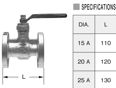
BM20K-FOLS (BALL VALVE TYPE)
