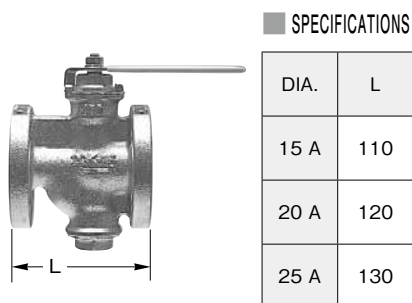
BM20K-FT (STRAINER BALL VALVE TYPE)
